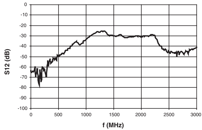
Figure 6-3. Reverse Transfer Function
