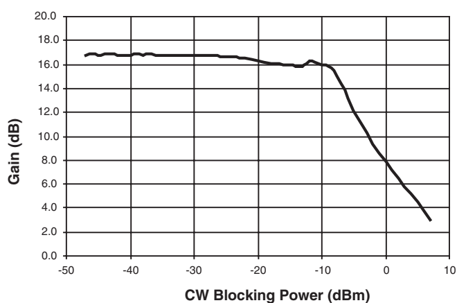
Figure 6-5. Gain versus Blocker at 1710 MHz (Compression)
