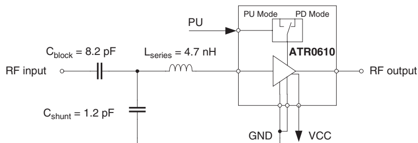
Figure 1-1. Block Diagram
